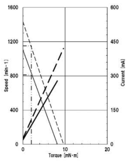
GEAR 100
