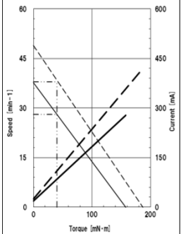
GEAR 300
